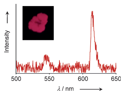
Figure 4. Emission spectra of [\text{Tb}_{0.99}\text{Eu}_{0.01}(\text{hfa})_3(\text{dpdp})]_n in the solid state at 500 K ( \lambda_{\text{ex}} = 380 nm, I_{\text{Eu}}/I_{\text{Tb}} = 10 ). Inset: Emission of [\text{Tb}_{0.99}\text{Eu}_{0.01}(\text{hfa})_3(\text{dpdp})]_n under UV (365 nm) irradiation at 500 K.
