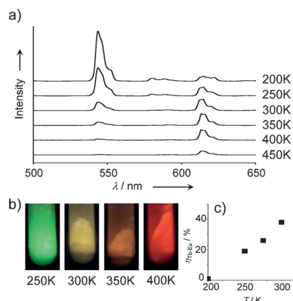
Figure 3. a) Temperature-dependent emission spectra of [\text{Tb}_{0.99}\text{Eu}_{0.01}(\text{hfa})_3(\text{dpdp})]_n in the solid state in the temperature range of 200–450 K ( \lambda_{\text{ex}} = 380 nm). b) Color pictures of [\text{Tb}_{0.99}\text{Eu}_{0.01}(\text{hfa})_3(\text{dpdp})]_n under UV (365 nm) irradiation, which show brilliant green, yellow, orange, and red emission. c) Temperature-dependence of the energy transfer efficiency ( \eta_{\text{Tb-Eu}} ).
