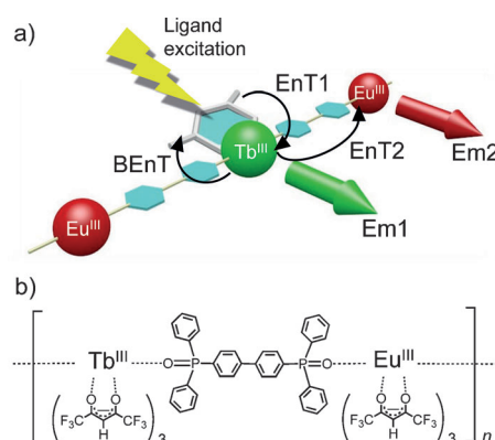
Figure 1. a) Energy transfer processes of the Eu III and Tb III coordination polymer (EnT: energy transfer, BEnT: energy back transfer, Em: emission). b) Chemical structure of [Ln(hfa) 3 (dpbb)] n (Ln = Eu, Tb).
